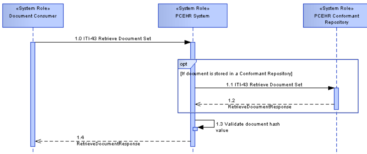
Figure 7 - ITI-43 Retrieve Document Set
