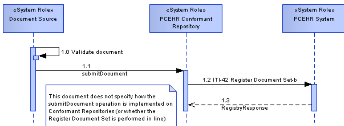
Figure 12 - ITI-42 Register Document Set-b
