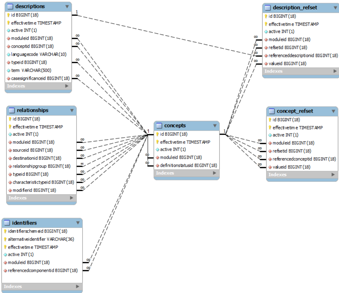
Figure 10: Schema Design for core SNOMED CT tables
