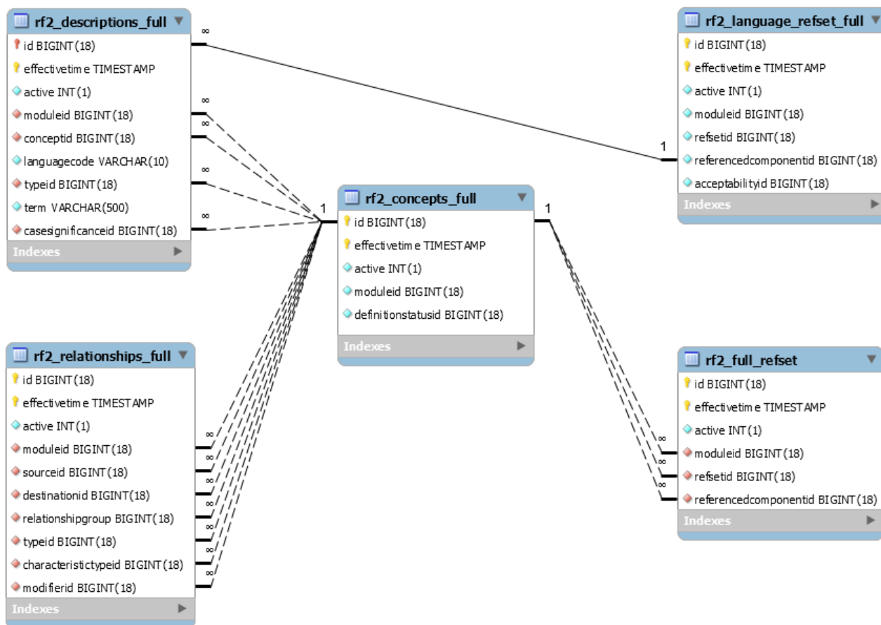
Figure 11: Schema Design for SNOMED CT-AU tables
