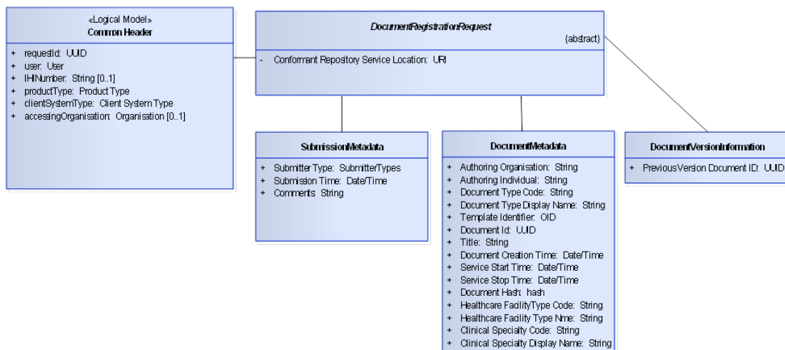
Figure 24 - DocumentRegistrationRequest
