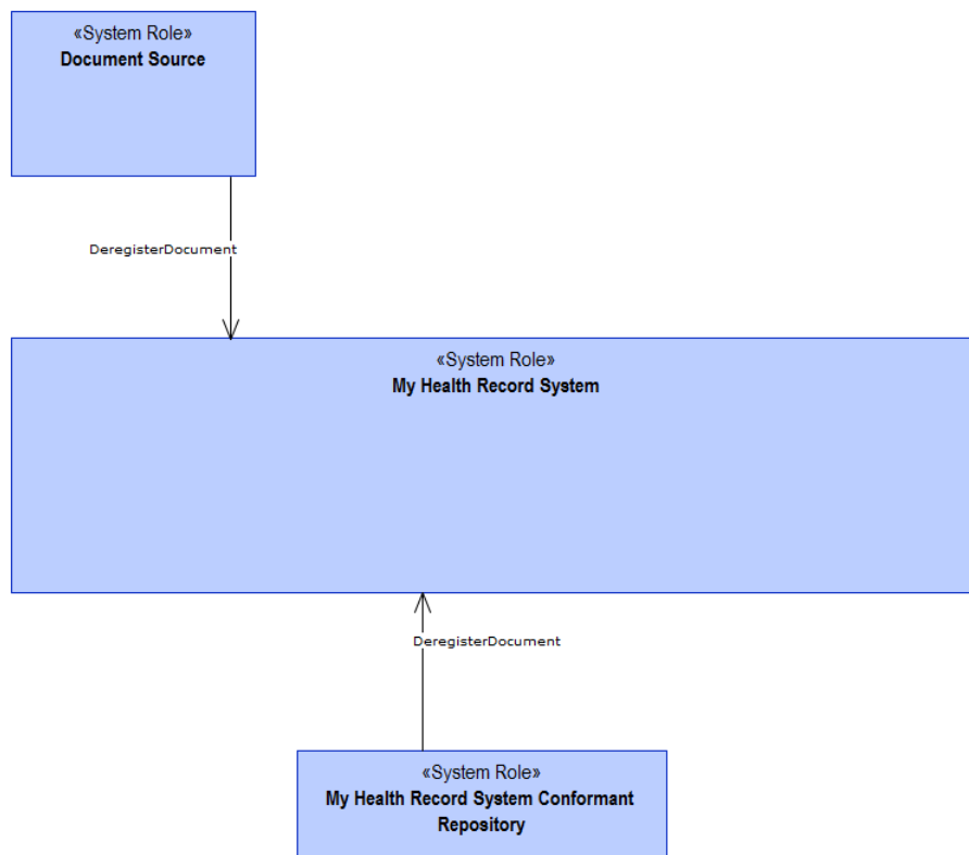
Figure 16 - deregisterDocument operation
