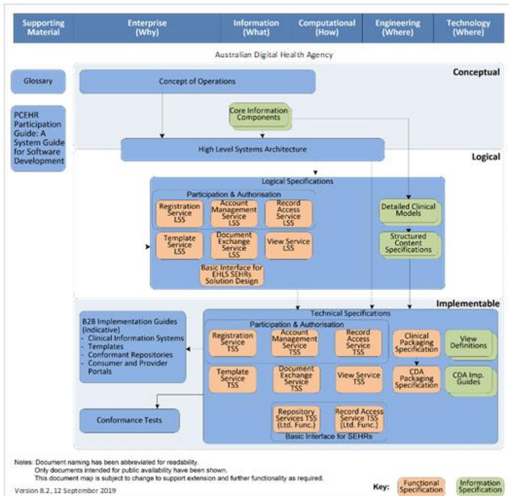
Figure 3 - Document map
