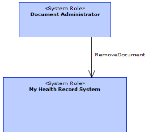
Figure 13 - removeDocument operation
