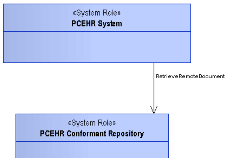
Figure 17 - retrieveRemoteDocument operation
