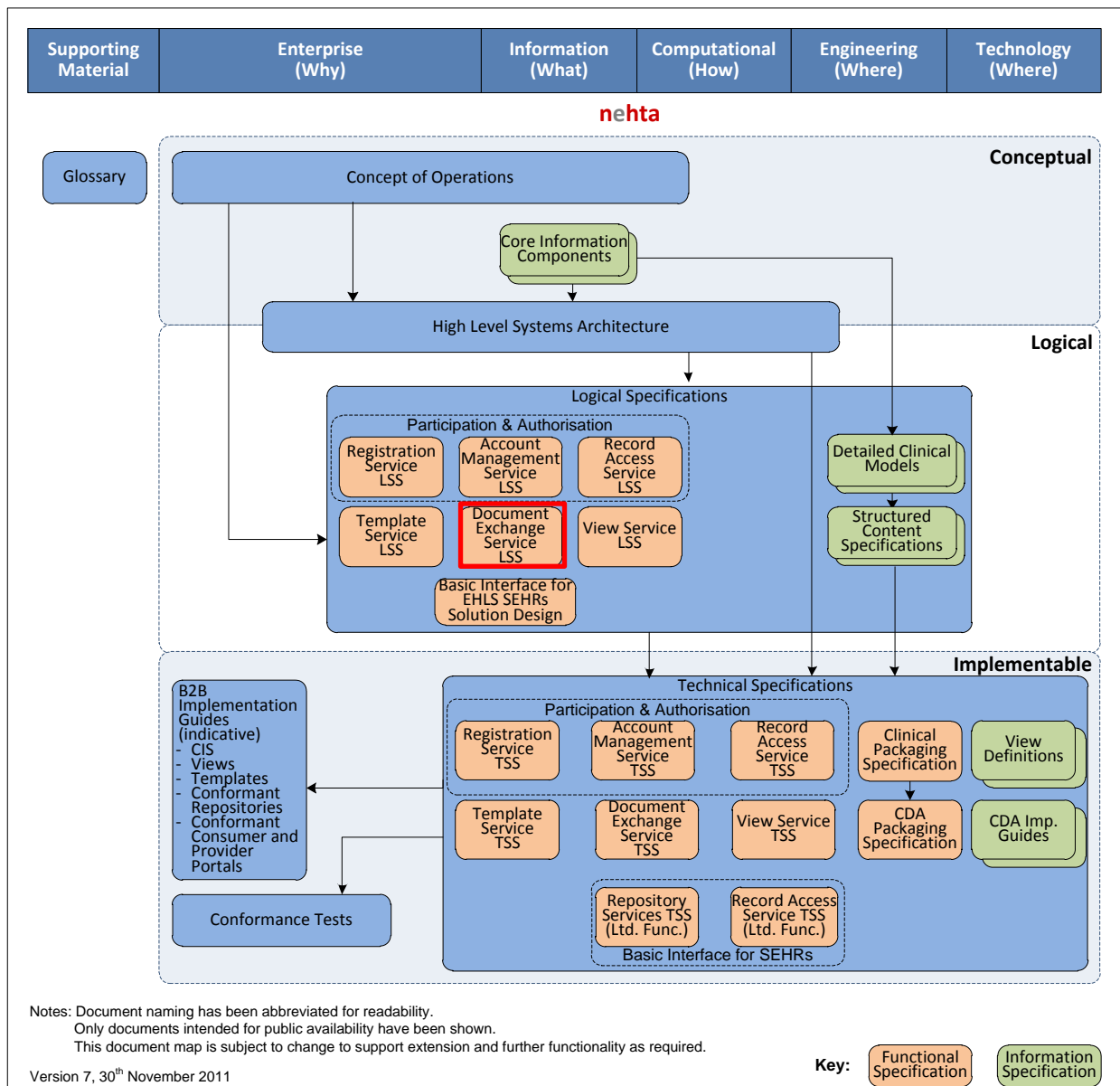
Figure 1 - Document Map
