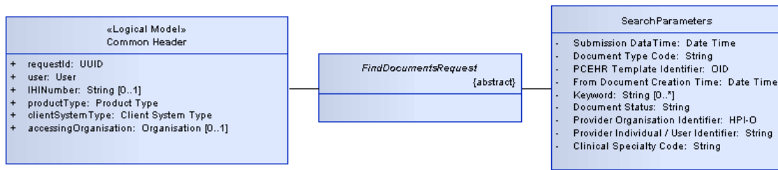
Figure 20 – FindDocumentsRequest
