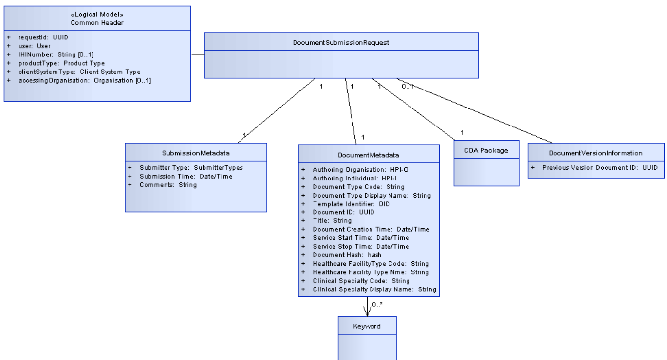
Figure 18 - DocumentSubmissionRequest
