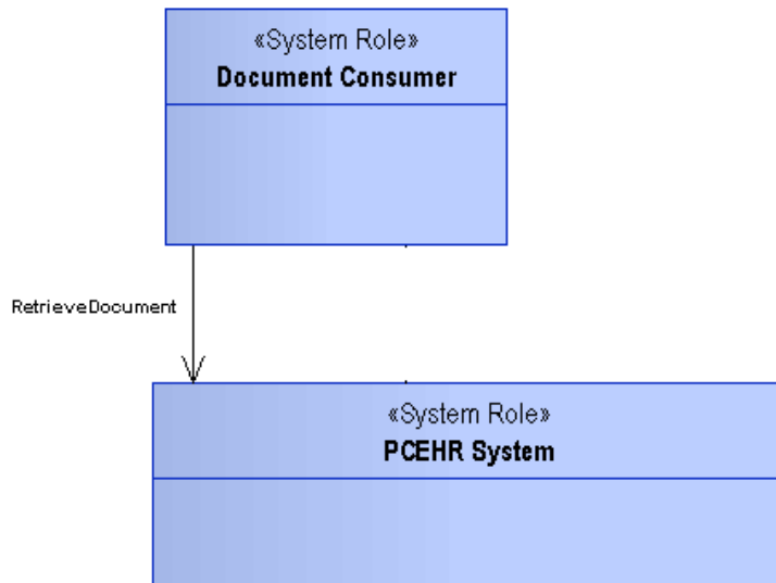
Figure 9 - retrieveDocument operation
