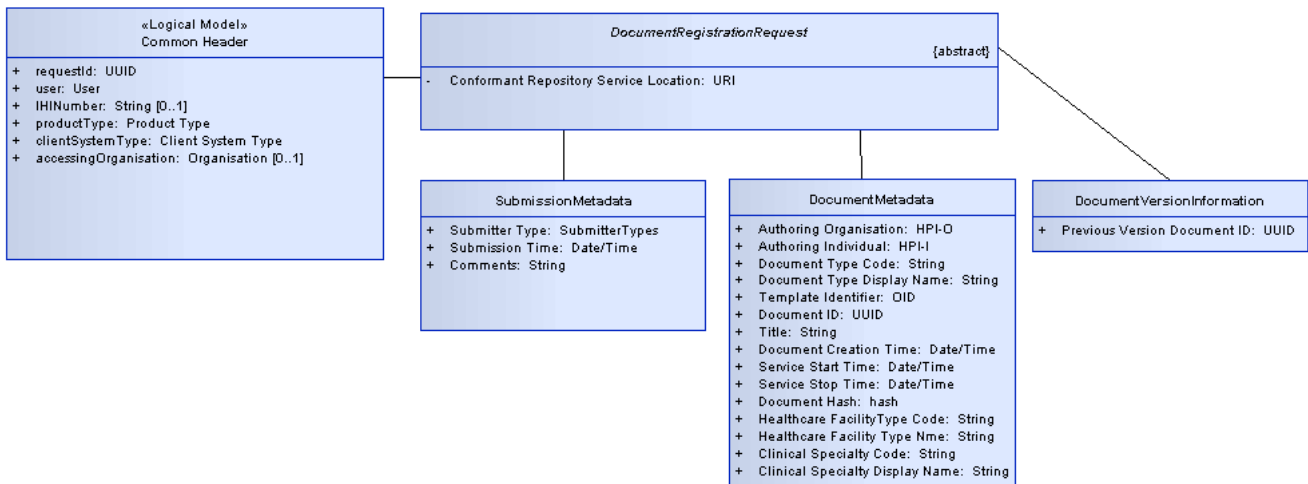
Figure 23 - DocumentRegistrationRequest
