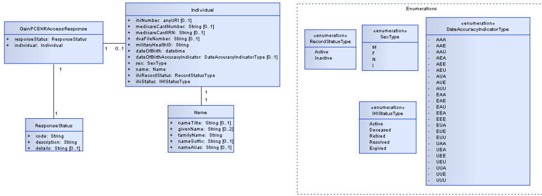
Figure 9 - GainPCEHRAccessResponse
