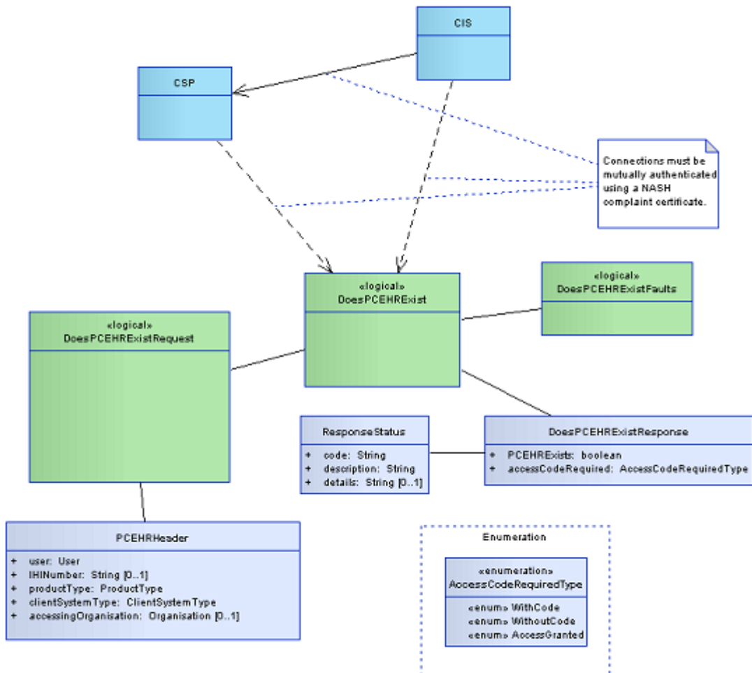
Figure 5 - doesPCEHRExist - Operation Data View
