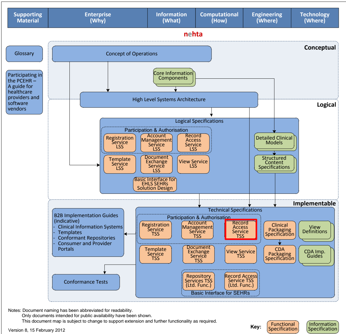
Figure 1 - Document Map
